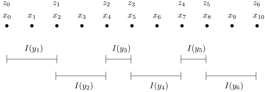
Figure 6: An interval representation for a poset P with no induced \mathbf{4} + \mathbf{1} . The forcing cycle C : x_0 \prec \cdots \prec x_{10} \parallel y_6 \parallel \cdots \parallel y_1 \parallel x_0 and the labeling determined from Table 5 show that wd_F(P) = 10/7 .
